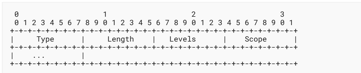
Figure 5: IS-IS Flooding Request TLV
