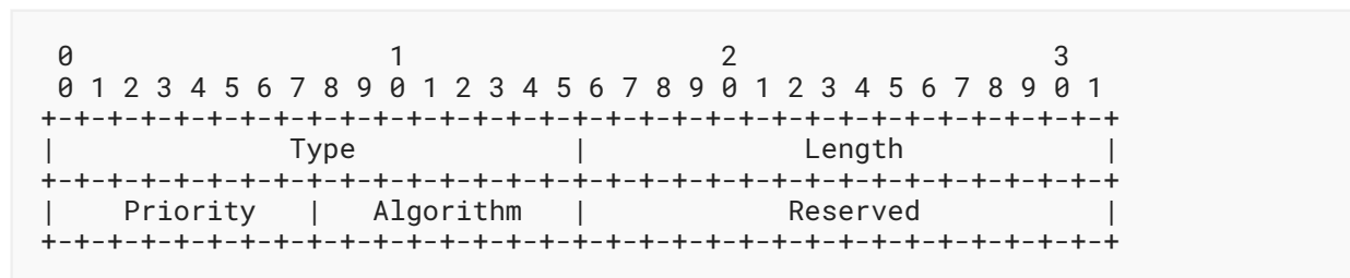
Figure 6: OSPF Area Leader Sub-TLV
