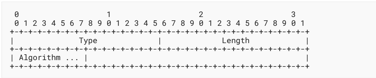
Figure 7: OSPF Dynamic Flooding Sub-TLV
