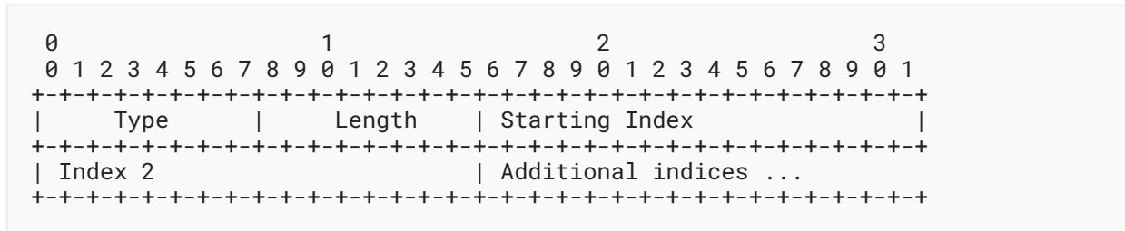
Figure 4: IS-IS Flooding Path TLV
