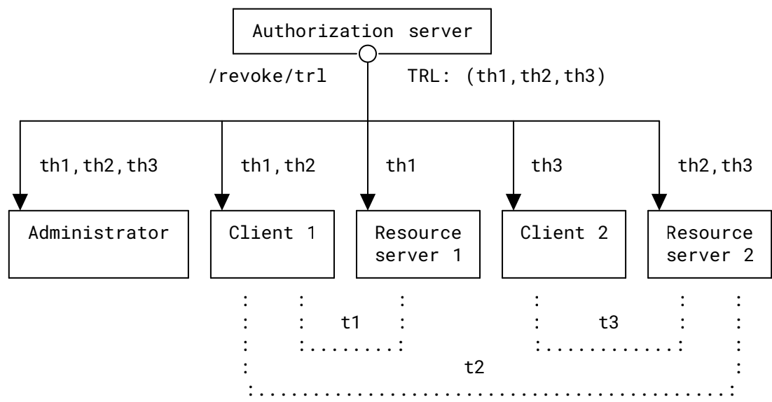
Figure 1: Protocol Overview
