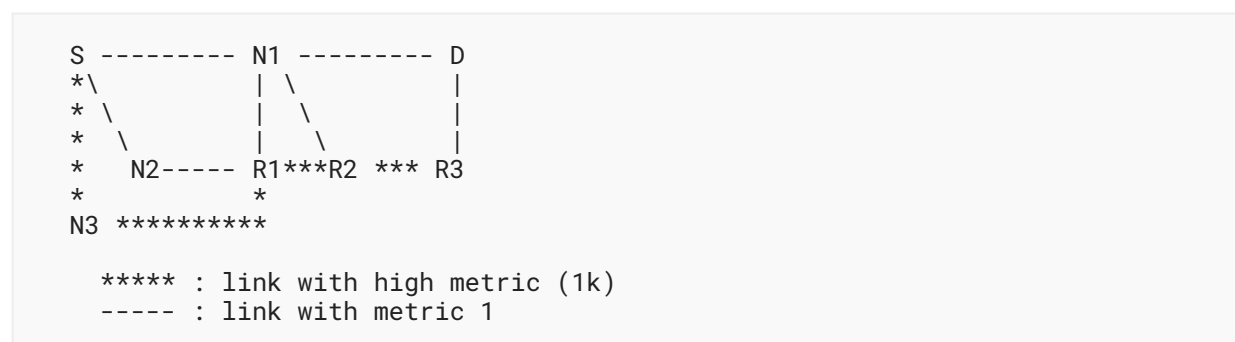
Figure 1: Sample Topology with TI-LFA
