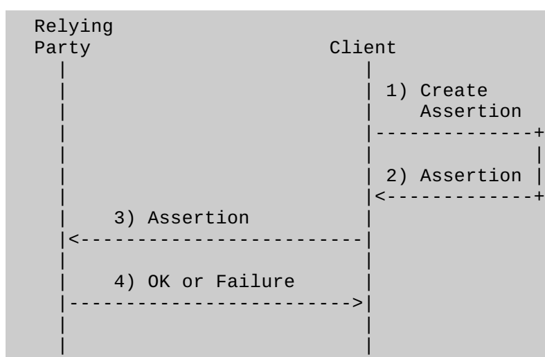
Figure 2: Self-Issued Assertion
