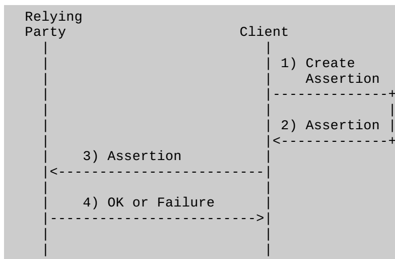
Figure 2: Self-Issued Assertion
